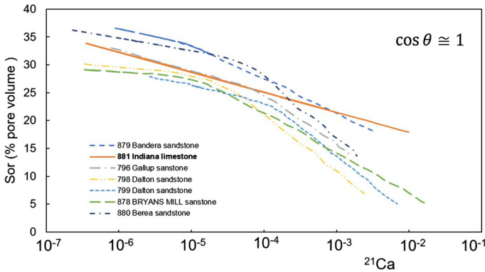
Fig. 10 CDC_{21} ( ^{21}\text{Ca} ) for various sandstones and one limestone from Abrams (1975, Fig. 5) illustrating the influence of viscosity contrast
