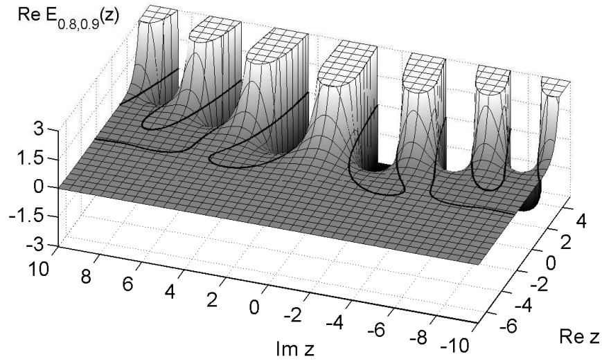
Fig. 2.1 Truncated real part of the generalized Mittag-Leffler function -3 \leq \operatorname{Re} E_{0.8,0.9}(z) \leq 3 for z \in \mathbb{C} with -7 \leq \operatorname{Re} z \leq 5 and -10 \leq \operatorname{Im} z \leq 10 . The solid line is defined by \operatorname{Re} E_{0.8,0.9}(z) = 0 .
