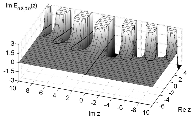
Fig. 2.2 Same as Fig. 2.1 for the imaginary part of E_{0.8,0.9}(z) . The solid line is \operatorname{Im} E_{0.8,0.9}(z) = 0 .
