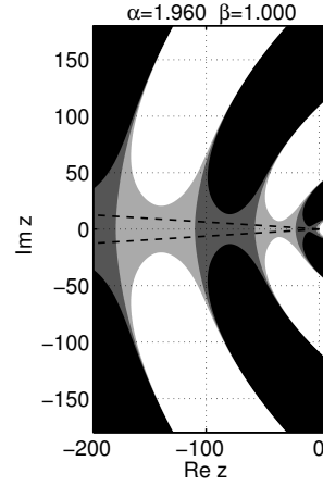
FIGURE 10. Contour plot for \operatorname{Re} E_{1.96,1}(z) . The dashed lines mark the wedge \mathbb{W}^+(\alpha\pi/2) . (The gray level coding is the same as in Figure 3)
