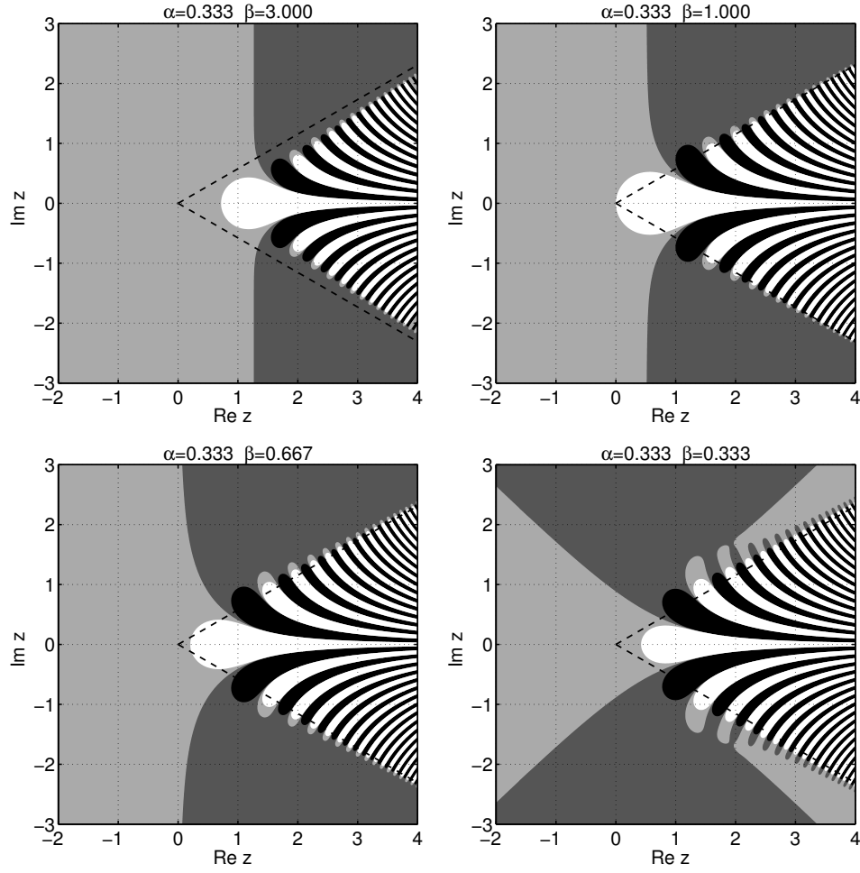
FIGURE 13. Contour plot for \operatorname{Re} E_{0.333, \beta}(z) with \beta = 3, 1, 2/3, 1/3 . The dashed lines mark the wedge \mathbb{W}^+(\alpha\pi/2) . (The gray level coding is the same as in Figure 3)
