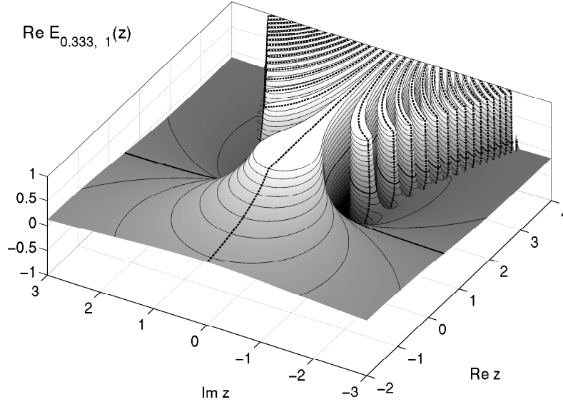
FIGURE 5. Truncated surface plot for \operatorname{Re} E_{0.333,1}(z) . Only the surface for -1 \leq \operatorname{Re} E_{0.333,1}(z) \leq 1 is shown. The contour lines \mathcal{C}_{0.333,1}^{\operatorname{Re}}(0) are shown as thick solid lines. The contour lines \mathcal{C}_{0.333,1}^{\operatorname{Im}}(0) are shown as thick dashed lines. Their intersections are zeros.
