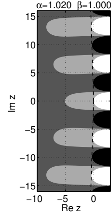
FIGURE 8. Contour plot for \operatorname{Re} E_{1.02,1}(z) . The dashed lines mark the wedge \mathbb{W}^+(\alpha\pi/2) . (The gray level coding is the same as in Figure 3)
