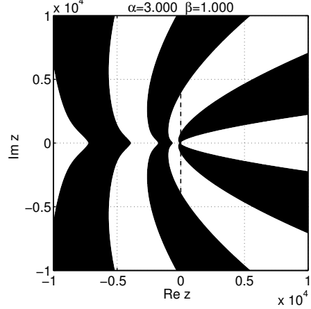
FIGURE 12. Contour plot for \text{Re } E_{3,1}(z) . The dashed lines mark the wedge \mathbb{W}^+(\alpha\pi/2) . (The gray level coding is the same as in Figure 3)
