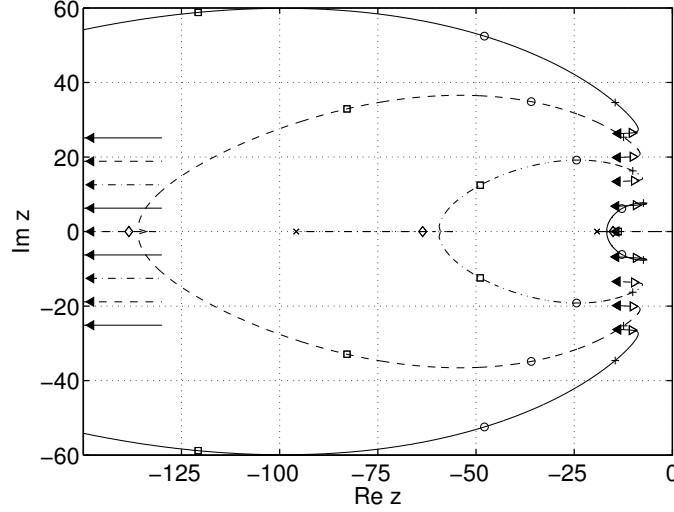
FIGURE 2. Locus of complex zeros z_k^0(\alpha) as functions of \alpha for k = \pm 1, \pm 2, \pm 3, \pm 4 for the the Mittag-Leffler function E_{\alpha,1}(z) in the range 1.00001 \leq \alpha \leq 1.9 . The line styles consecutively label k = \pm 1 (solid) k = \pm 2 (dashed) k = \pm 3 (dash-dotted), k = \pm 4 (solid). The symbols mark \alpha = 1.00001 (triangle left filled) \alpha = 1.001 (triangle right) \alpha = 1.1 (plus) \alpha = 1.3 (circle) \alpha = 1.5 (square), and \alpha = 1.7 (diamond) \alpha = 1.9 (cross). The arrows on the left indicate the asymptotic locations z_k^0(1) = 2k\pi in the limit \alpha \rightarrow 1 from above.
