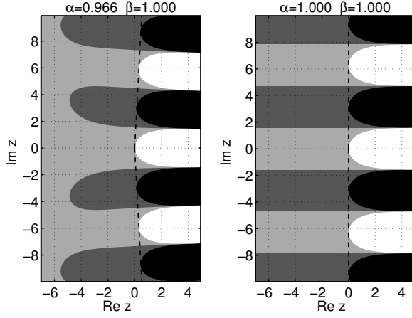
FIGURE 7. Contour plots for \operatorname{Re} E_{0.966,1}(z) and \operatorname{Re} E_{1,1}(z) . The dashed lines mark the wedge \mathbb{W}^+(\alpha\pi/2) . (The gray level coding is the same as in Figure 3)
