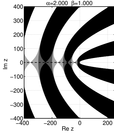
FIGURE 11. Contour plot for \text{Re } E_{2,1}(z) . The dashed lines mark the wedge \mathbb{W}^+(\alpha\pi/2) . (The gray level coding is the same as in Figure 3)
