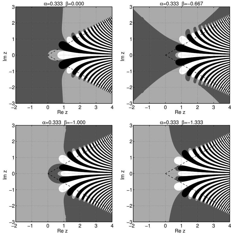
FIGURE 14. Contour plot for \text{Re } E_{1/3, \beta}(z) for \beta = 0, -2/3, -1, -4/3 . The dashed lines mark the wedge \mathbb{W}^+(\alpha\pi/2) . (The gray level coding is the same as in Figure 3)
