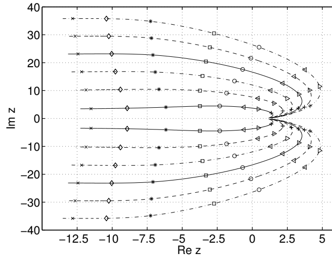
FIGURE 1. The lines trace out the locus of complex zeros z_k^0(\alpha) as functions of \alpha for k = -5, \dots, 6 for the the Mittag-Leffler function E_{\alpha,1}(z) in the range 0.1 \leq \alpha \leq 0.99995 . The line styles consecutively label k = 0, 1 (solid) k = -1, 2 (dashed) k = -2, 3 (dash-dotted), k = -3, 4 (solid) k = -4, 5 (dashed) and k = -5, 6 (dash-dotted). The symbols mark \alpha = 0.5 (plus), \alpha = 0.7 (triangle right), \alpha = 0.8 (triangle left), \alpha = 0.9 (circle), \alpha = 0.95 (square), \alpha = 0.99 (asterisk), \alpha = 0.999 (diamond), and \alpha = 0.9999 (cross).
