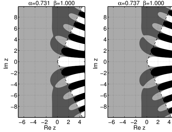
FIGURE 6. Contour plot for \operatorname{Re} E_{0.731,1}(z) and \operatorname{Re} E_{0.737,1}(z) , before and after the first osculation estimated to occur at \alpha \approx 0.734375 \pm 0.000015 . The dashed lines mark the wedge \mathbb{W}^+(\alpha\pi/2) . (The gray level coding is the same as in Figure 3)
