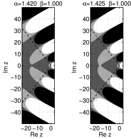
FIGURE 9. Contour plot for \operatorname{Re} E_{1.420,1}(z) and \operatorname{Re} E_{1.425,1}(z) before and after the osculation estimated to occur at \alpha \approx 1.42215 \pm 0.00005 . The dashed lines mark the wedge \mathbb{W}^+(\alpha\pi/2) . (The gray level coding is the same as in Figure 3)
