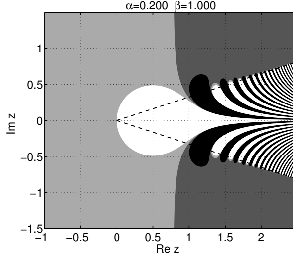
FIGURE 4. Contour plot for \operatorname{Re} E_{0.2,1}(z) . The dashed lines mark the wedge \mathbb{W}^+(\alpha\pi/2) . (The gray level coding is the same as in Figure 3)
