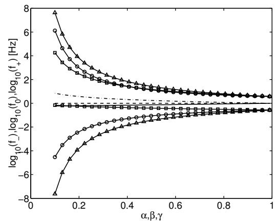
FIGURE 2. Location of the frequency of the maximum f_0 , frequency f_- of lower half width and frequency f_+ of upper half width of the imaginary part of Cole-Cole, Kohlrausch and Cole-Davidson susceptibility functions as function of the respective stretching exponents \alpha , \beta , \gamma . The upper and lower half width frequencies f_\pm are indicated by solid lines connected with symbols (Cole-Cole susceptibility function ( \Delta ), Kohlrausch susceptibility ( \circ ), Cole-Davidson ( \square )). The location of the maximum of the imaginary part is indicated by a dashed line for the Cole-Cole function, by a solid line without symbols for the Kohlrausch function and by a dashdotted line for the Cole-Davidson function. The relaxation time is always \tau = 1 .
