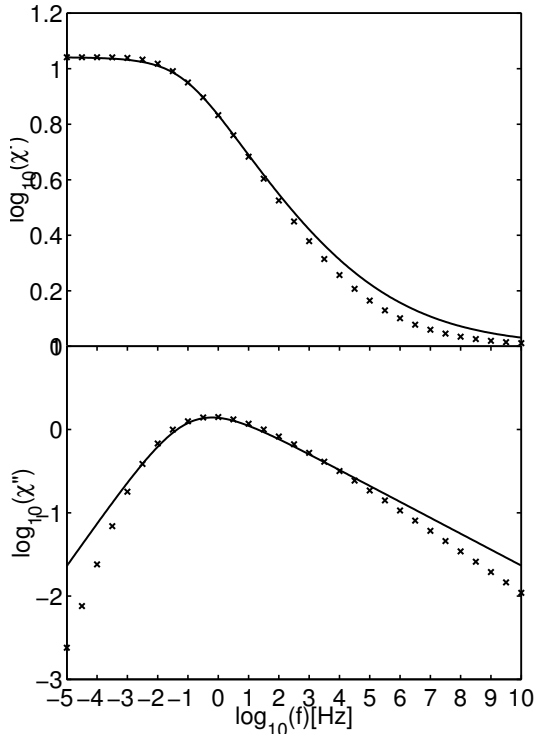
FIGURE 1. Comparison of the Havriliak-Negami fit (solid line) with \alpha = 0.5164 , \gamma = 0.3706 and \tau_H = 10 for a Kohlrausch susceptibility ( \times ) with \beta = 0.25 and \tau_\beta = 1 . The values were taken from Ref. [7], page 7310, Table I. In all cases \chi_\infty = 1 and \chi_0 = 10 .
