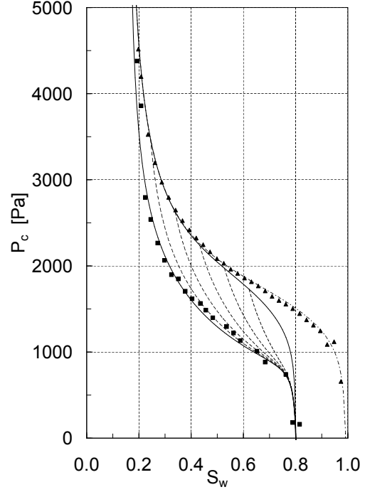
FIGURE 2. Hysteresis loop for capillary pressure P_c as function of water saturation S_w as in Fig. 1. The imbibition scanning curves start from the secondary drainage curve. Parameters and line styles are identical to those in Figure 1.
