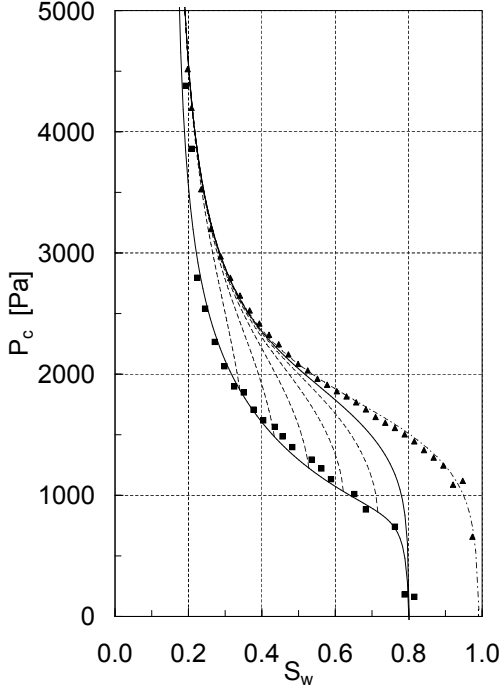
FIGURE 1. Hysteresis loop and drainage scanning curves for capillary pressure P_c as function of water saturation S_w fitted to experimental data obtained for a water wet medium grained sand of porosity \phi = 0.34 . The primary drainage curve is the dash-dotted line. The main hysteresis loop is the solid line. The dashed lines are drainage scanning curves. All eight curves have the same parameters: S_{w,dr} = 0.15 , S_{\odot,im} = 0.19 , \alpha = 0.52 , \beta = 0.90 , \gamma = 1.5 , \delta = 3.5 , \eta_2 = 4 , \eta_4 = 3 , \Pi_a = 1620 Pa, \Pi_b = 25 Pa, and P_2^* = 2500 Pa P_4^* = 400 Pa. The five scanning curves start from the boundary imbibition curve at S_w = 0.3, 0.4, 0.5, 0.6, 0.7 .
