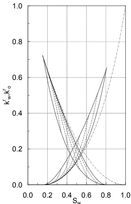
FIGURE 3. Hysteresis loop and drainage scanning curves for relative permeabilities k_w^r, k_o^r as function of water saturation S_w . Parameters and line styles are identical to those for capillary pressure in Figures 1 and 2. Here \kappa_w = \kappa_o = 0 and the parameters R_1^*, R_3^* are chosen such that R_1^* = 2\phi^2\mu_w/k and R_3^* = 2\phi^2\mu_o/k .
