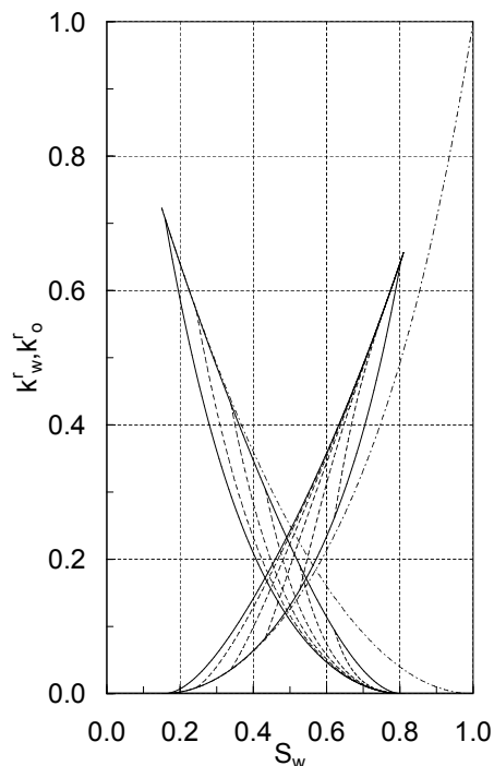
FIGURE 4. Same as Figure 3 with imbibition scanning curves starting from the secondary drainage curve. Parameters and line styles are identical to those in Figure 3.
