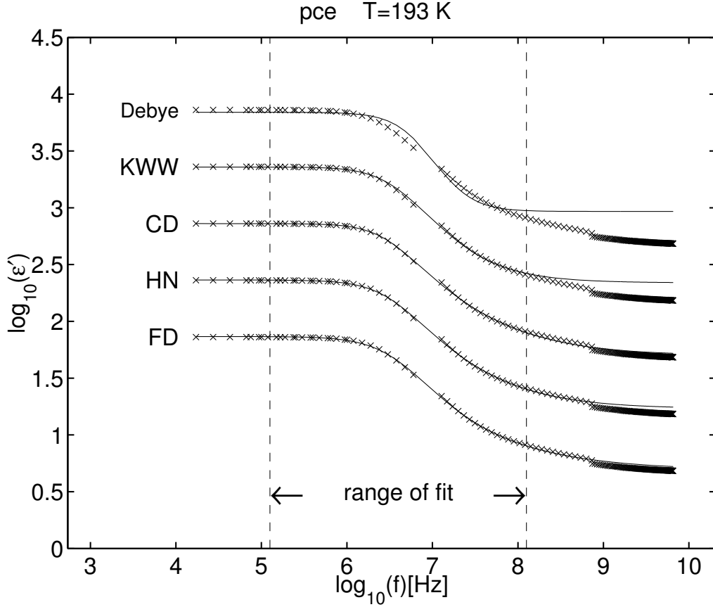
FIGURE 1. Five different fits to the real part \varepsilon'(f) of the complex dielectric function of propylene carbonate at T = 193K as a function of frequency f . Experimental data represented by crosses are from Ref. [56]. The fitting functions corresponds to an exponential (Debye), stretched exponential (KWW), Cole-Davidson [57, 58] Havriliak-Negami [59, 60] and the fractional dynamics (FD) relaxation from (40). The range over which the data were fitted is indicated by dashed vertical lines in the figure. For clarity the data were displaced vertically by half a decade each. The original location of the data corresponds to the curve labelled FD.
