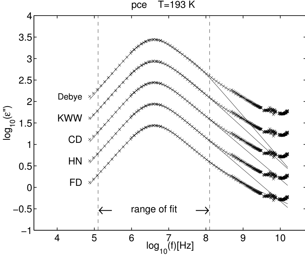
FIGURE 2. Five different fits as in Figure 1 for the imaginary part \varepsilon''(f) of the complex dielectric function of propylene carbonate at T = 193K as a function of frequency f .
