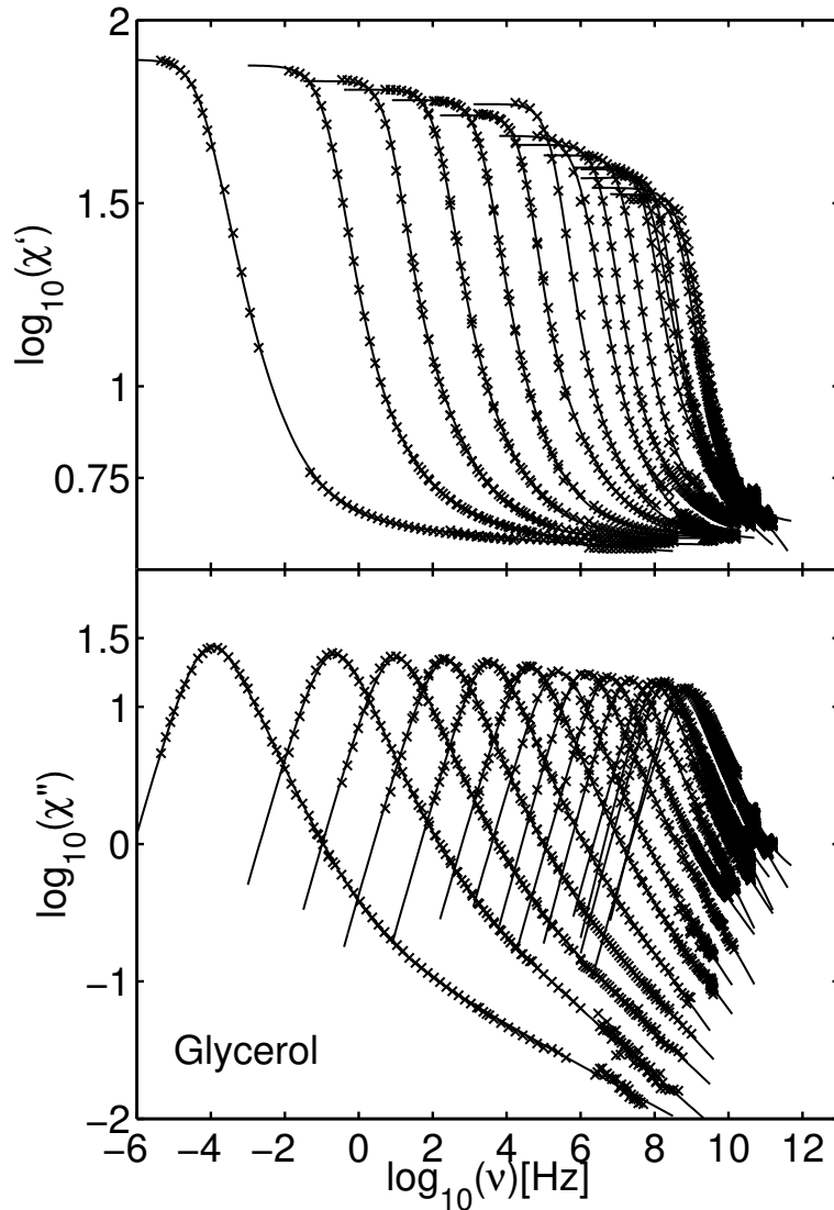
FIGURE 3. Separate fits for real part (upper figure) and imaginary part (lower figure) of the complex dielectric susceptibility \chi(\nu) = \chi'(\nu) + i\chi''(\nu) of glycerol for temperatures T = 323, 303, 295, 289, 273, 263, 253, 243, 234, 223, 213, 204, 195, 184 K (from right to left) as function of frequency \nu (from [54]). The experimental data are taken from Ref. [56], the fit uses a generalized composite fractional relaxation model. For details see [54].
