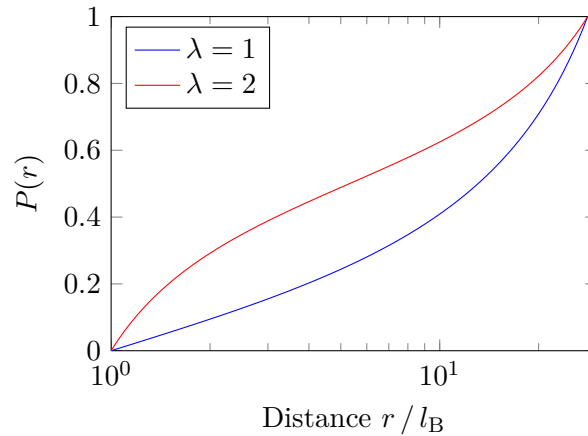
Figure 1: Poisson-Boltzmann solution for the charge distribution P(r) over radius r for the default parameters.
